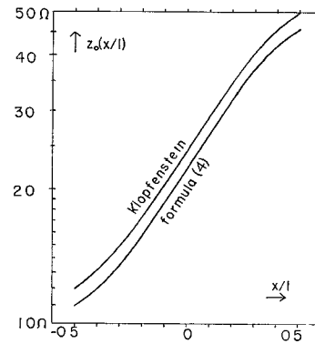
Fig. 1. Impedance taper.
